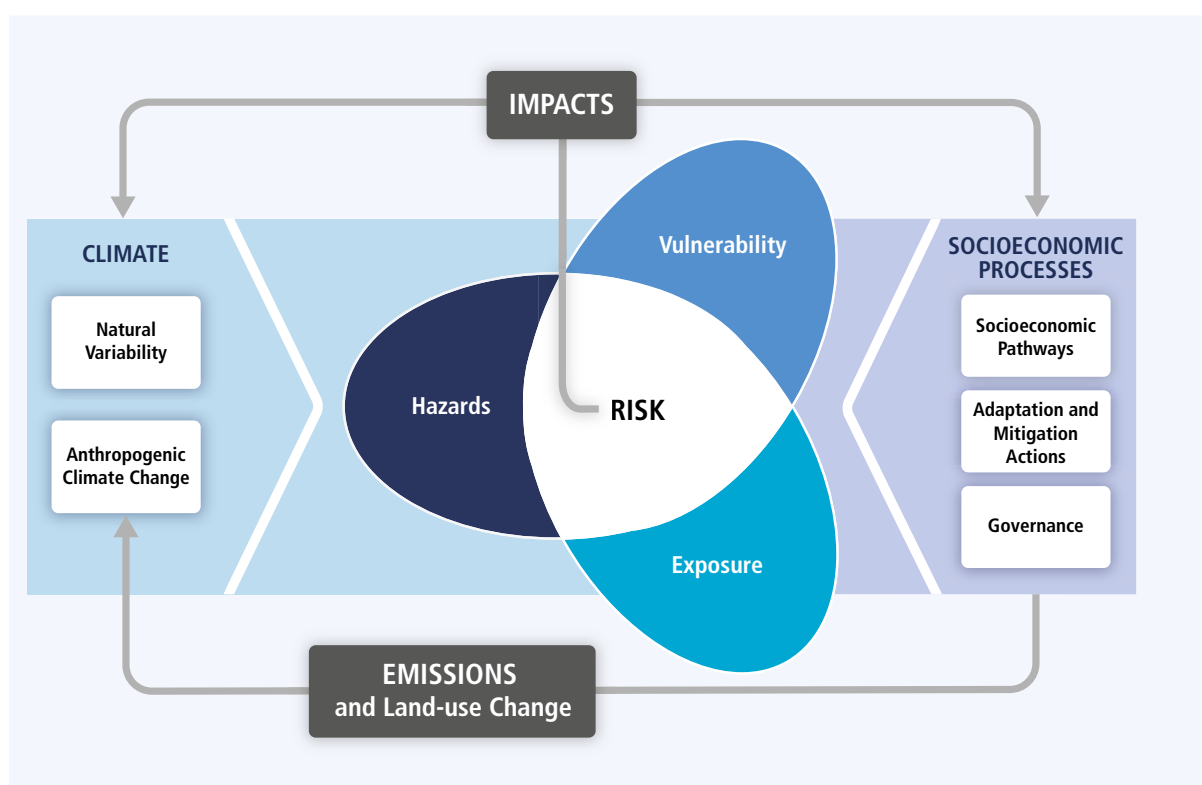
Figure 7: The IPCC AR5 conceptual framework with risk at the centre (IPCC, 2014).
