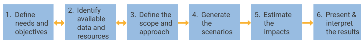
Figure 8: Physical Climate Risk Assessment Process (World Bank, 2019).
