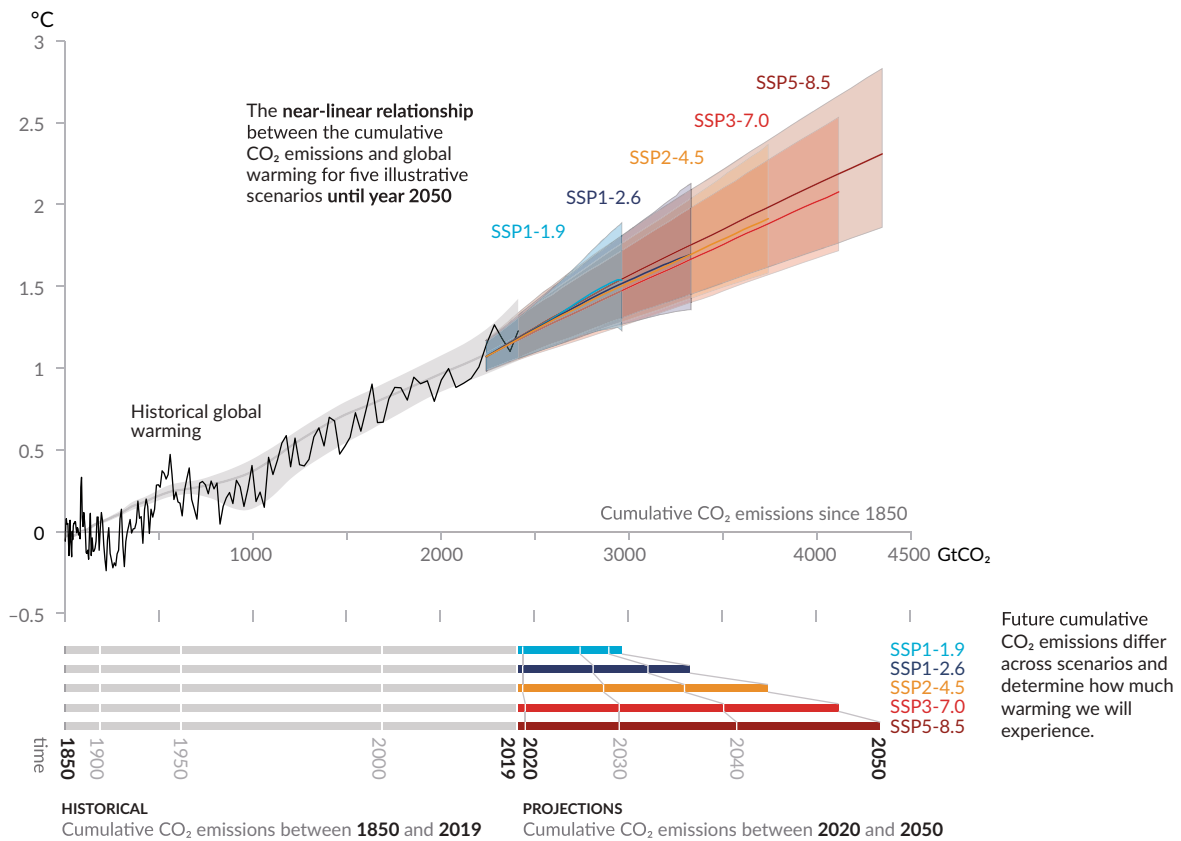
Figure 6: Every tonne of CO 2 emissions adds to global warming (IPCC, 2021).
