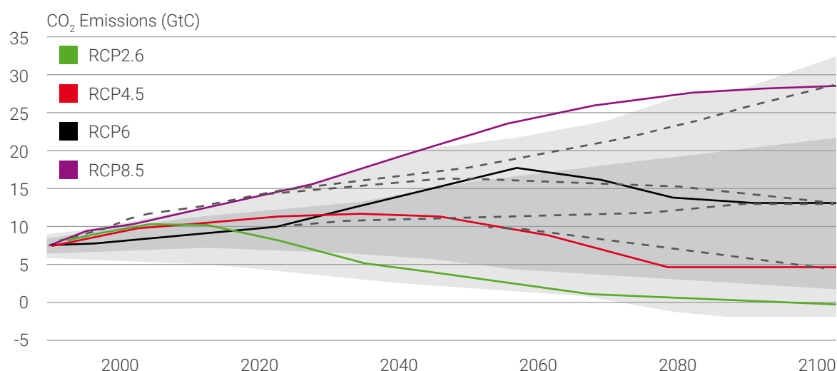
Figure 5: Emissions of carbon dioxide across the RCPs (van Vuuren et. al. , 2011).
